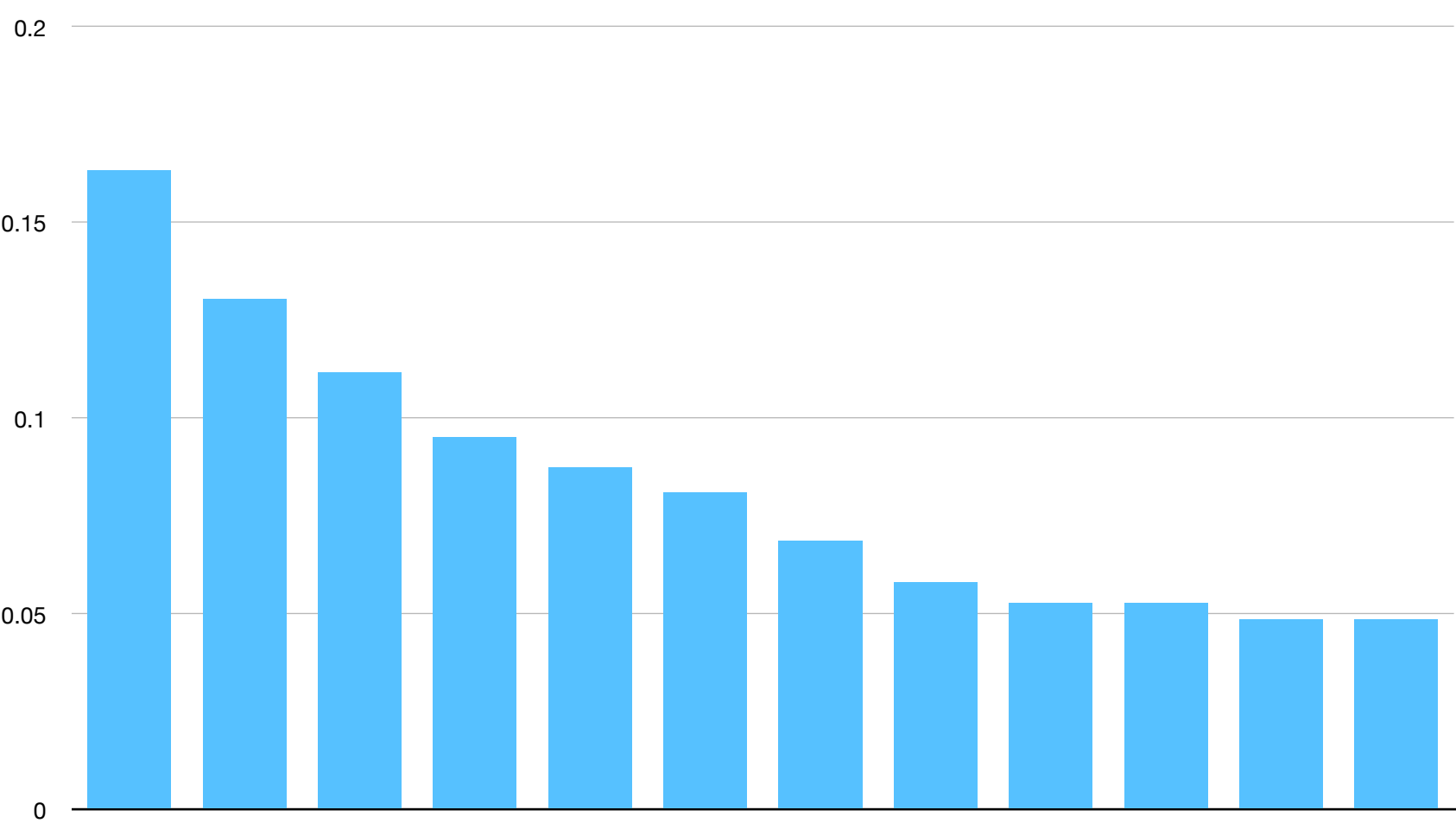
Fig B.5 - Relative SNR Ignoring Brightest Star (Max SNR=4.6)
