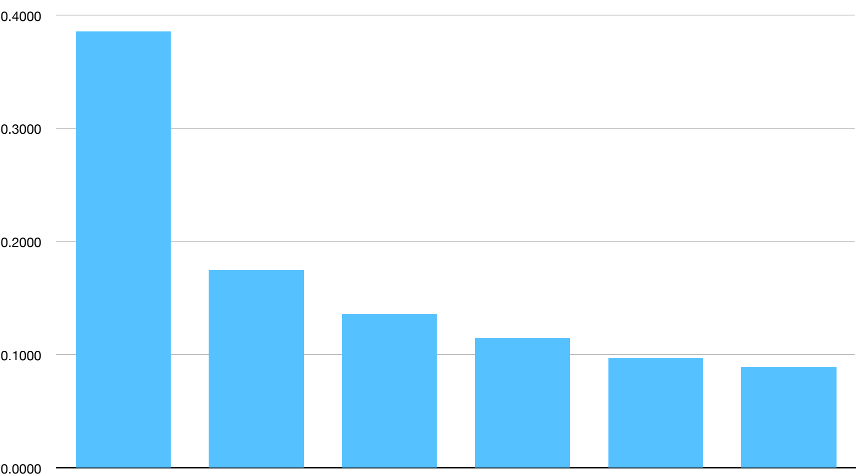
Fig B.4 - Relative SNR for 6 Guide Stars (Max SNR=10)
