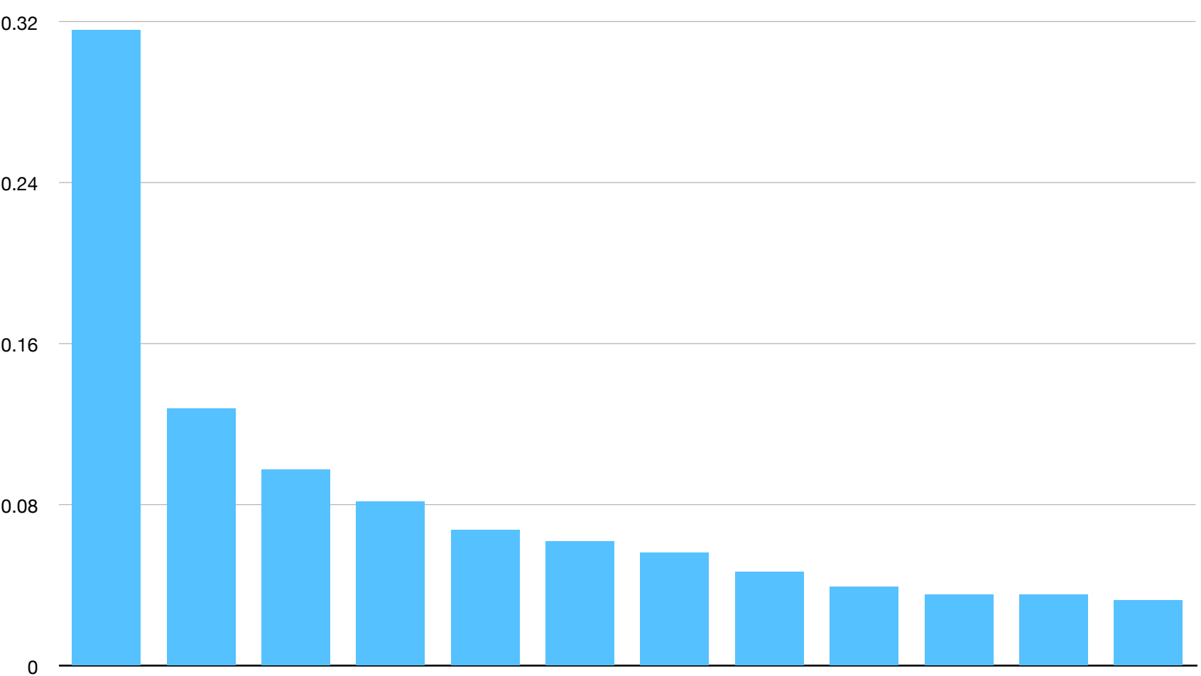
Fig B.3 - Relative SNR for 12 Guide Stars (Max SNR=4)
